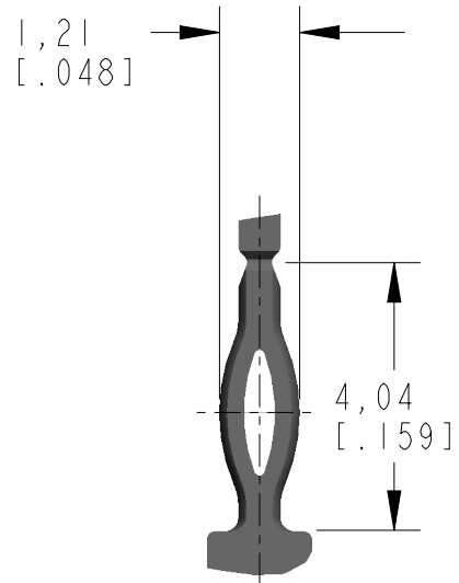
DETAIL "A"
