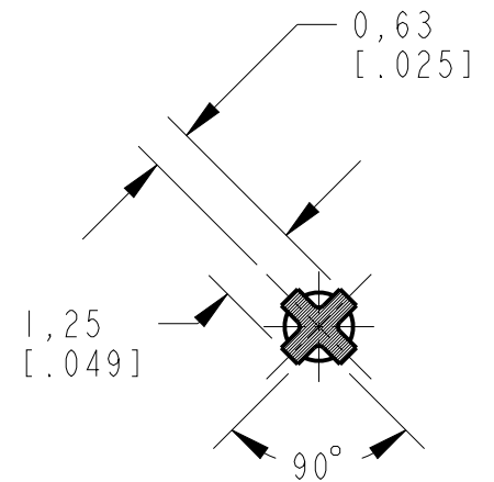
COMPLIANT DETAIL
